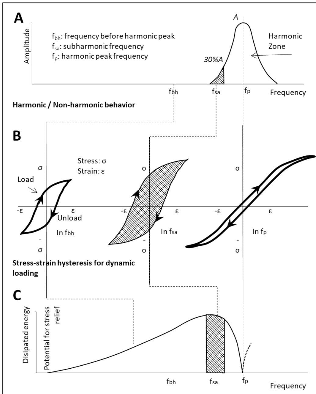
Figure 2: Frequency vs. hysteresis energy dissipation, per cycle Source: [4]
