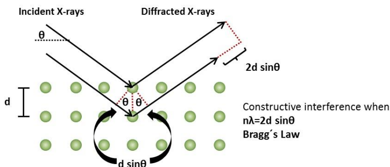
Figure 4: Principle of X-ray diffraction. Source: Anton Paar [8]
